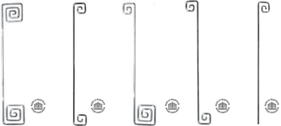
Art. 1146/1 \varnothing 12 x 12 mm H 1000 mm L 185 mm Art. 1146/2 \varnothing 12 x 12 mm H 1000 mm L 110 mm Art. 1146/3 \varnothing 12 x 12 mm H 1000 mm L 280 mm Art. 1146/4 \varnothing 12 x 12 mm H 1000 mm L 205 mm Art. 1146/5 \varnothing 12 x 12 mm H 1000 mm L 110 mm
