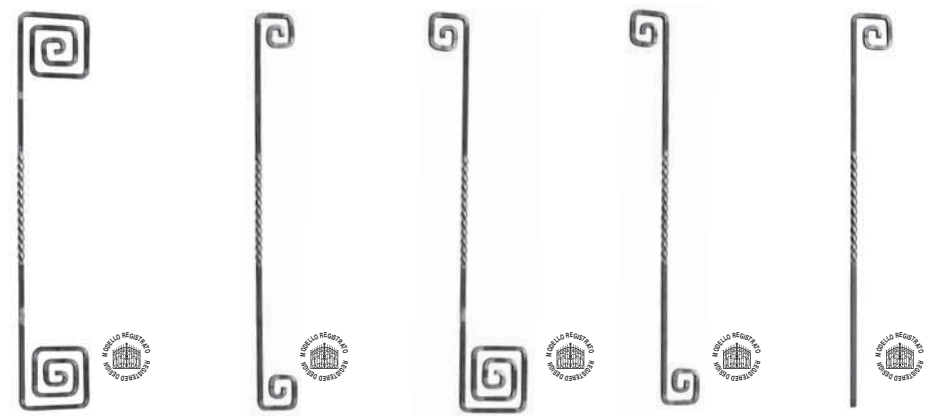
Art. 1147/1 \varnothing 12 x 12 mm H 1000 mm L 185 mm Art. 1147/2 \varnothing 12 x 12 mm H 1000 mm L 110 mm Art. 1147/3 \varnothing 12 x 12 mm H 1000 mm L 280 mm Art. 1147/4 \varnothing 12 x 12 mm H 1000 mm L 205 mm Art. 1147/5 \varnothing 12 x 12 mm H 1000 mm L 110 mm
