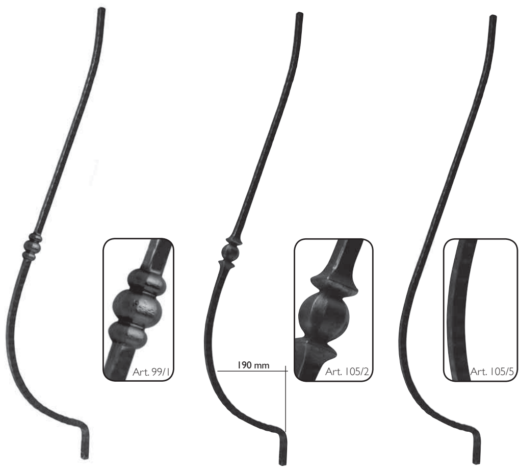
Art. 1783/8 Ø 12 x 12 mm H 1000 mm
