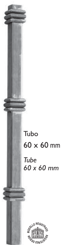
Art. 1207/1 H 1200 mm L 85 mm Art. 1246/1 H 1000 mm L 85 mm
