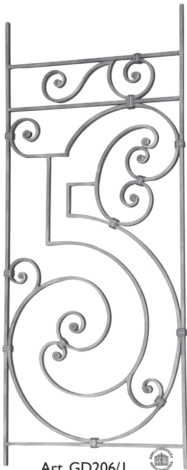
Art. GD206/1 □ 14 x 8 mm H 1000 mm L 420 mm
