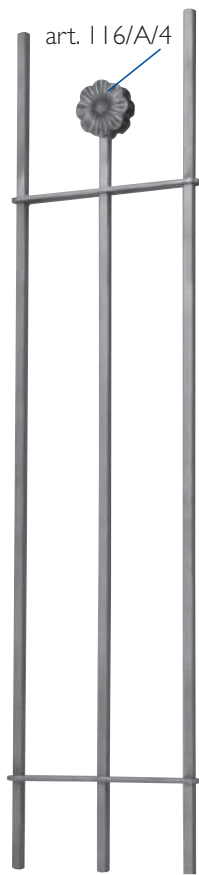
Art. GD26/1 Ø 12 x 12 mm H 1000 mm L 235 mm
