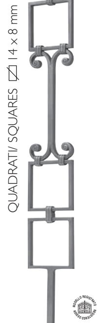
Art. GDI84/2 Ø 14 x 14 mm H 1000 mm L 115 mm
