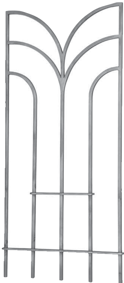
Art. GD68/I \Phi 12 x 12 mm H 1000 mm L 460 mm
