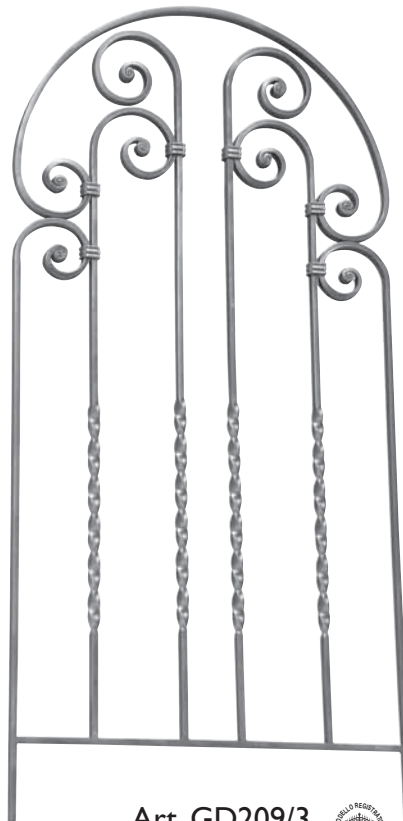
Art. GD209/3 □ 14 x 8 mm H 1000 mm L 480 mm
