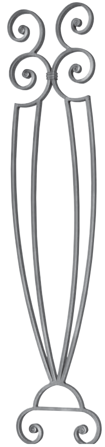
Art. GDI75/7 □ 14 x 8 mm H 1000 mm L 200 mm
