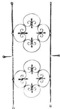
staffe/stafs 10 x 10 mm Art. 162/4 φ 10 x 5 mm H 1030 mm L 580 mm
