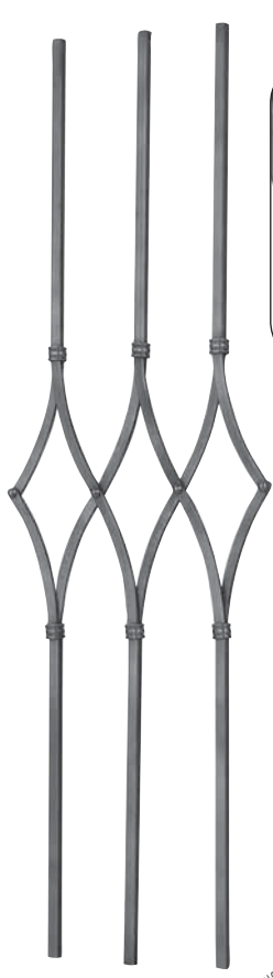
Art. GD21/I Ø 12 x 12 mm H 1000 mm L 315 mm
