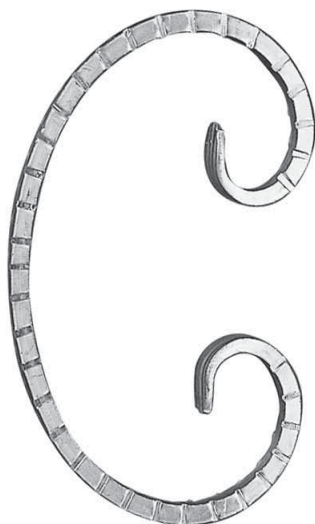
Art. 770/15 ∅ 12 x 6 mm H 150 mm L 105 mm
